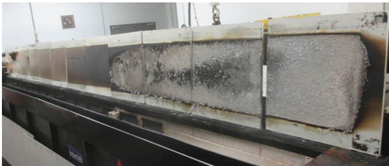
Photo No. 4 Exposed Surface of the Test Specimen (Post-test)
